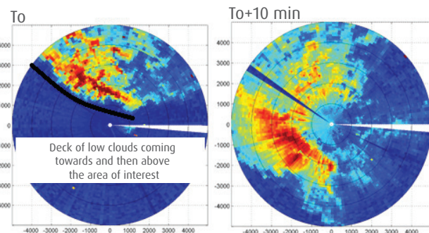
WINDCUBE 200S full PPI at low elevation Relative attenuated backscatter measurement
