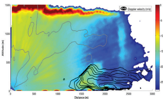
WINDCUBE 100S RHI cross section of a thunderstorm gust front Ipswich region, Queensland, Australia (Dec. 27 th . 2013)
